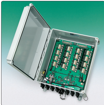
● Geokon Model 8032 Multiplexer (MUX).
