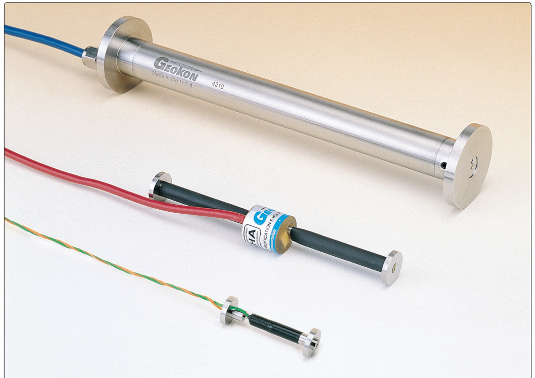
• Model 4202 (front), Model 4200 (center) and Model 4210 (rear) Concrete Embedment Strain Gages.
